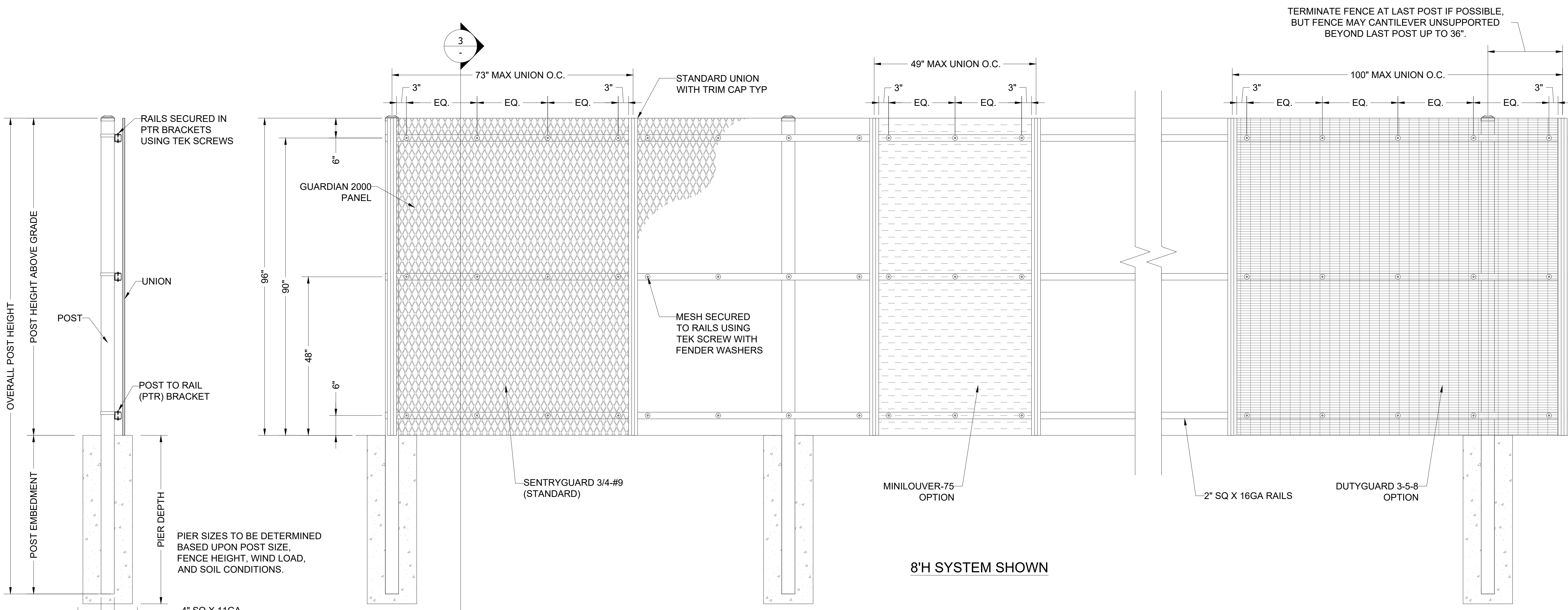
1 GUARDIAN 2000 TYPICAL ELEVATION SCALE: NTS
