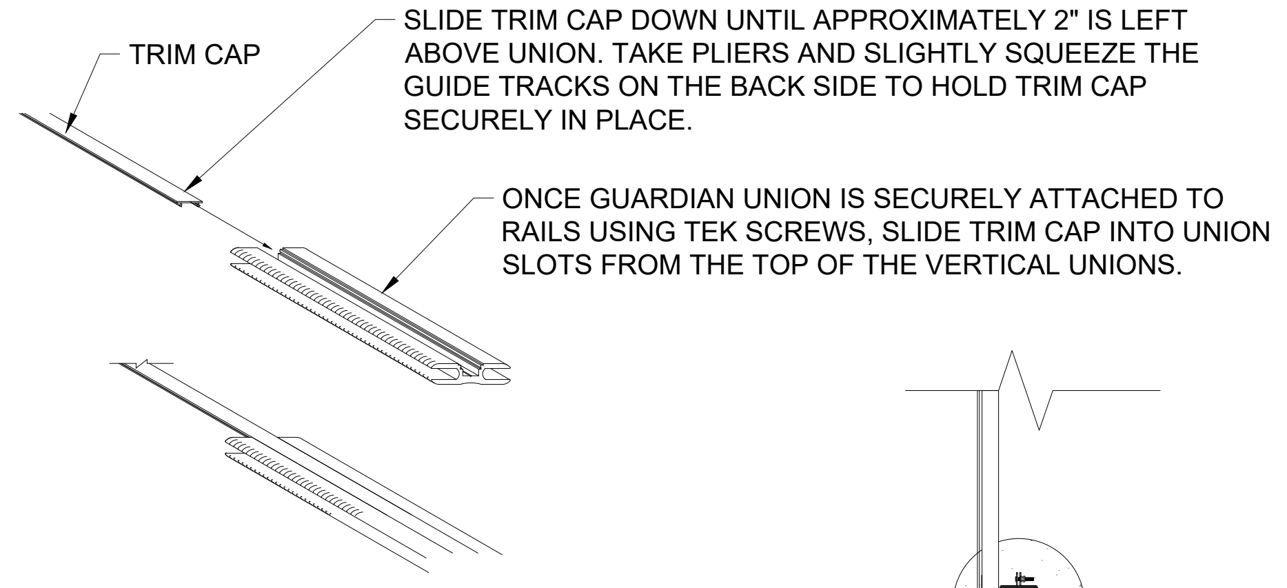
2 STANDARD UNION TRIM CAP DETAIL SCALE: NTS
